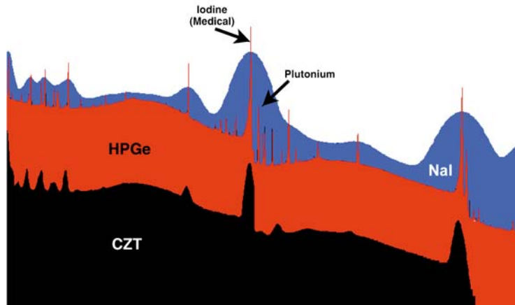
Figure 1. Radioactive Material Fingerprints. Same Material Viewed with Three Types of Technology.
